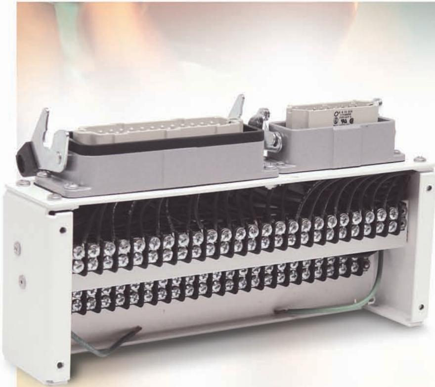
MJBW Series Mold Junction Box
